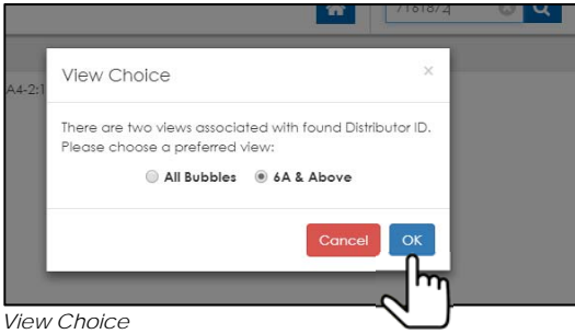
View Choice
