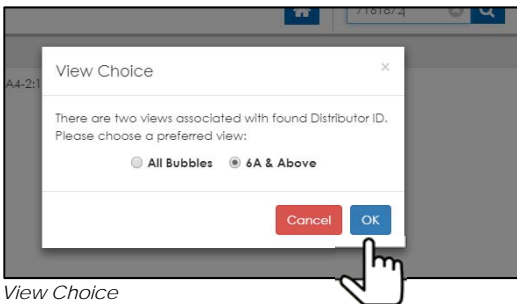
View Choice
