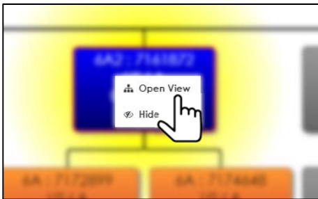
Open View
